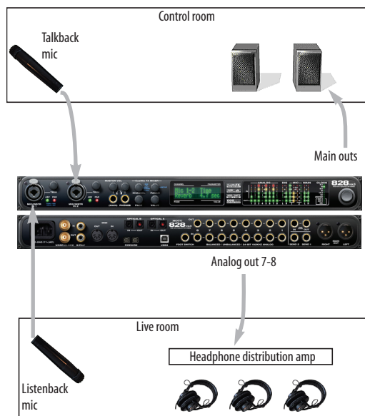
Figure 10-25: Typical hardware setup for Talkback and Listenback.
