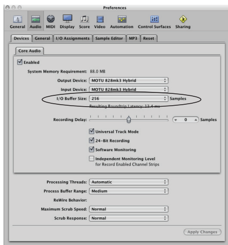
Figure 9-5: In Logic Pro or Logic Express, go to the Audio Driver preferences to access the Buffer Size option shown above.
