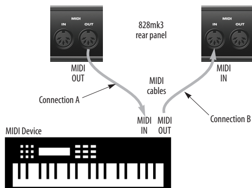
Figure 3-10: Connecting a MIDI device to the 828mk3.
