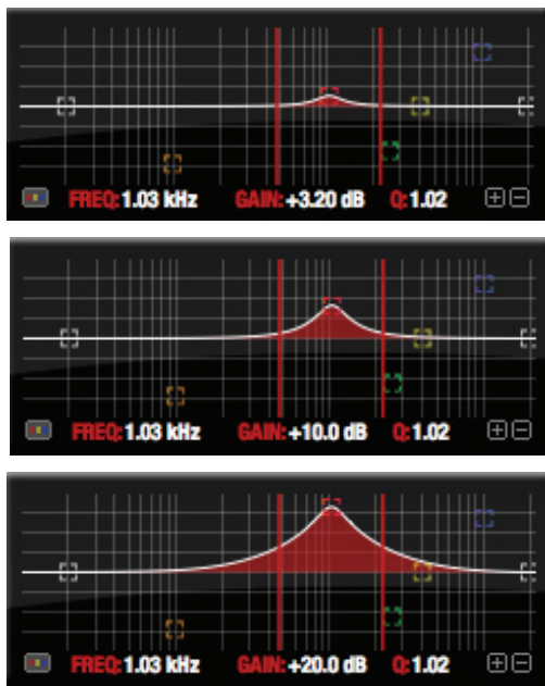
Figure 10-13: Type I EQ filter style.
