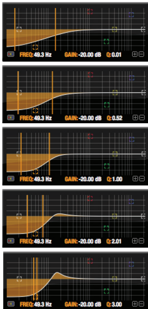
Figure 10-17: Shelf filter Q parameter overshoot.
