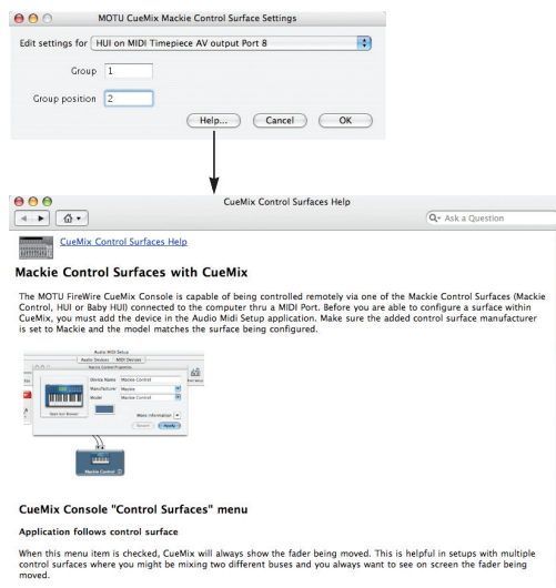
Figure 10-58: Refer to the extensive on-line help for details about configuring CueMix FX for operation with your control surface product.
