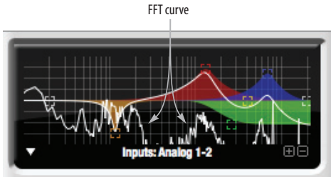
Figure 10-30: FFT display.
