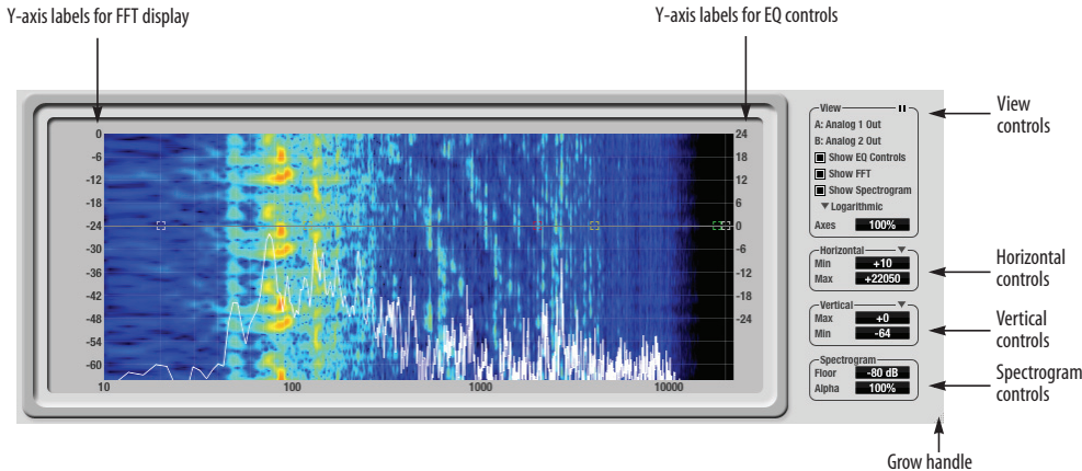
Figure 10-29: Full window filter display.
