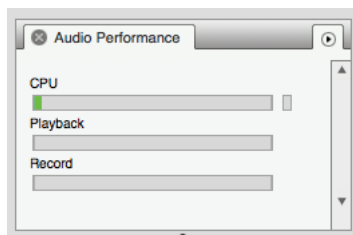
Figure 9-6: When adjusting the buffer size to reduce monitoring latency, watch the 'processor' meter in Digital Performer or AudioDesk's Performance Monitor. If you hear distortion, or if the Performance meter is peaking, try raising the buffer size.
