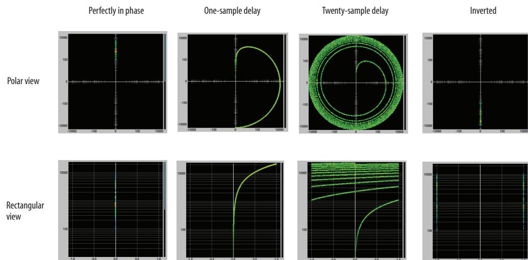
Figure 10-56: Two identical audio streams in the Phase Analysis.
