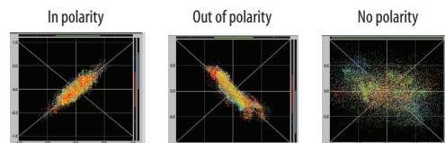
Figure 10-48: Checking polarity in a stereo signal with the X-Y Plot.
