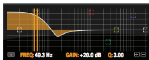
Figure 10-18: Overshoot when low shelf boost is applied.
