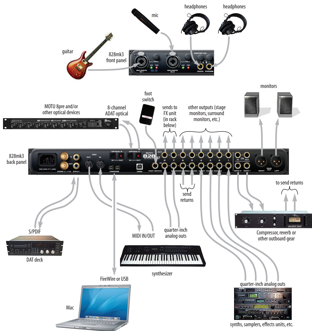
Figure 3-12: A typical 828mk3 studio setup.
