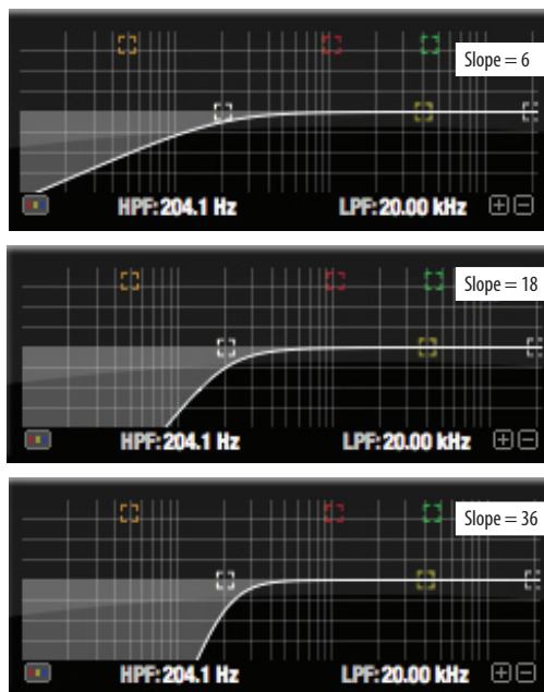
Figure 10-20: The low pass filter with three example slope settings.
