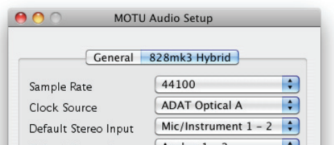
Figure 3-9: Resolving the 828mk3 to an optical device.
