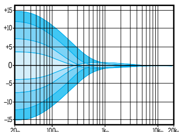
LM-3204 Lo shelving EQ \pm 15 dB boost/cut.
