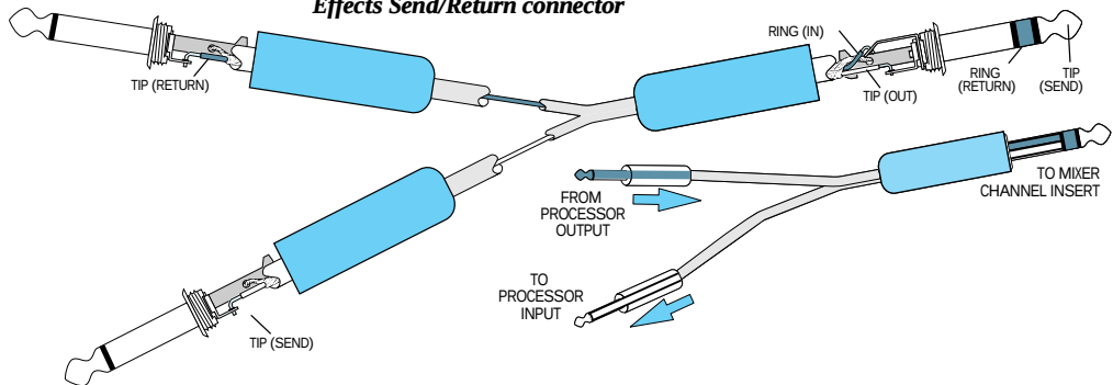
Effects Send/Return connector
