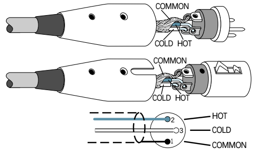
Balanced XLR Connectors
