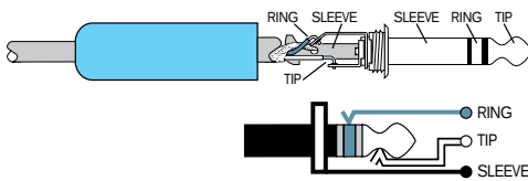
Tip/Ring/Sleeve (TRS) Plug
