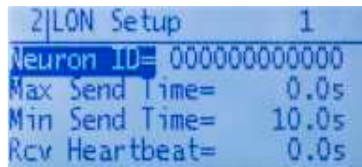
Figure 11: LON Set-Up Menu
