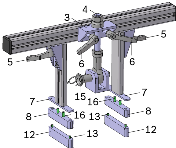
Figure 3: Support bar
