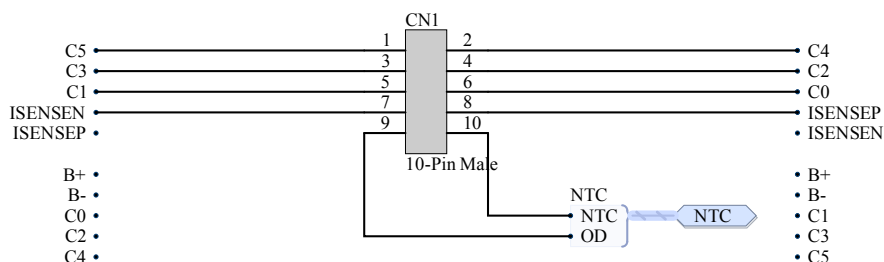
Figure 7. CN1 connector
