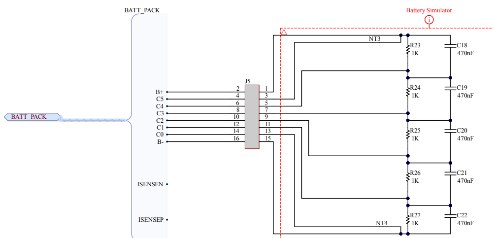
Figure 4. Power supply connector and battery simulator
