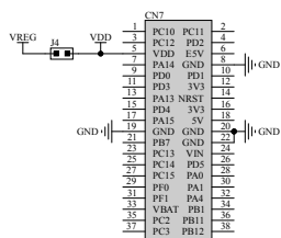
Figure 22. STEVAL-L99615C expansion board schematic (5/5)
