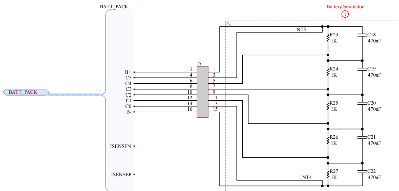
Figure 22. STEVAL-L99615C expansion board schematic (5/5)
