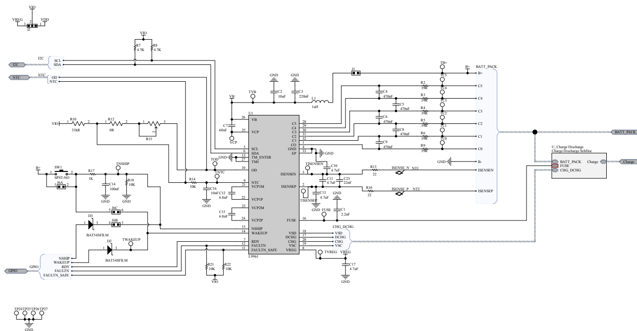
Figure 19. STEVAL-L99615C expansion board schematic (2/5)
