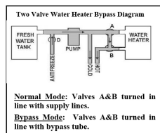
Two Valve Water Heater Bypass
