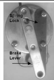
Brake lever released
