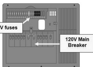
Load Center Panel w/120 volt Main breaker – load center appearance and configuration may vary by model
