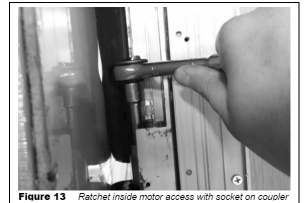
Figure 13 Ratchet inside motor access with socket on coupler
