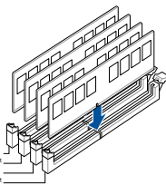
DIMM_A1 DIMM_A2 1st DIMM_B1 DIMM_B2 1st
