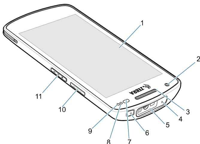
Figure 1 Front View
