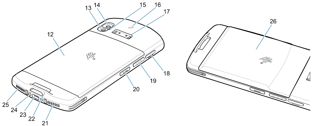
Figure 2 Rear View
