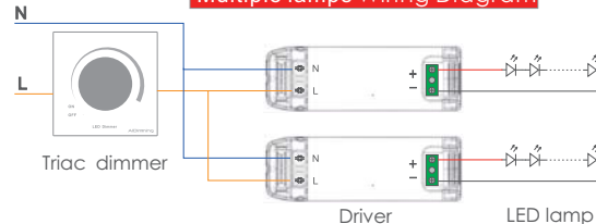
Multiple lamps Wiring Diagram
