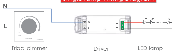
Single lamp Wiring Diagram
