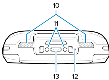
Figure 3 Bottom View
