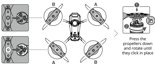
Match the propellers to motors
