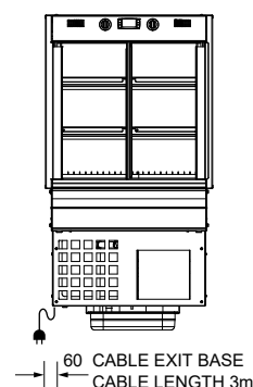
REAR ELEVATION
