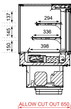
SECTION VIEW
