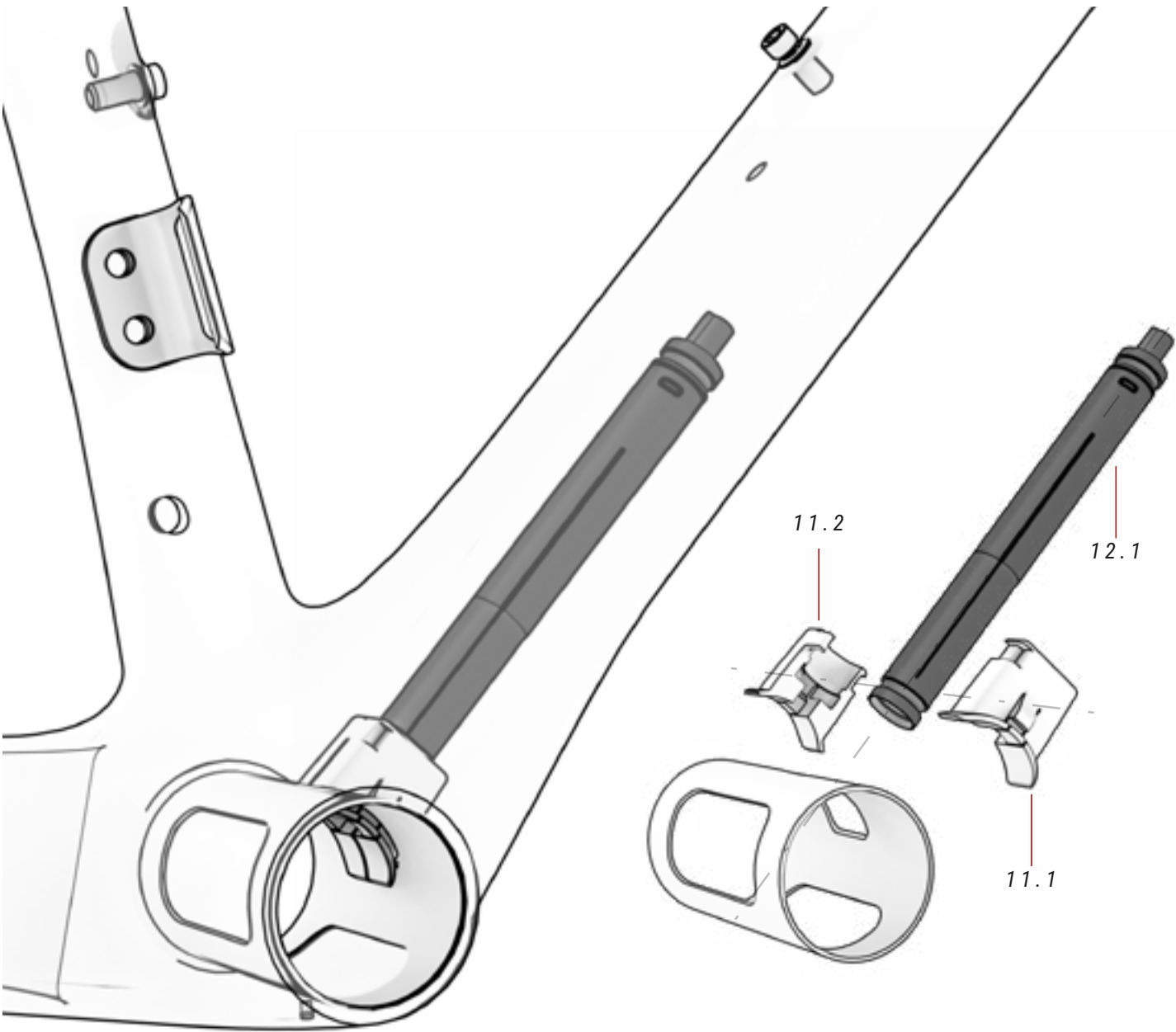
11 DI2 BOTTOM BRACKET HOLDER
