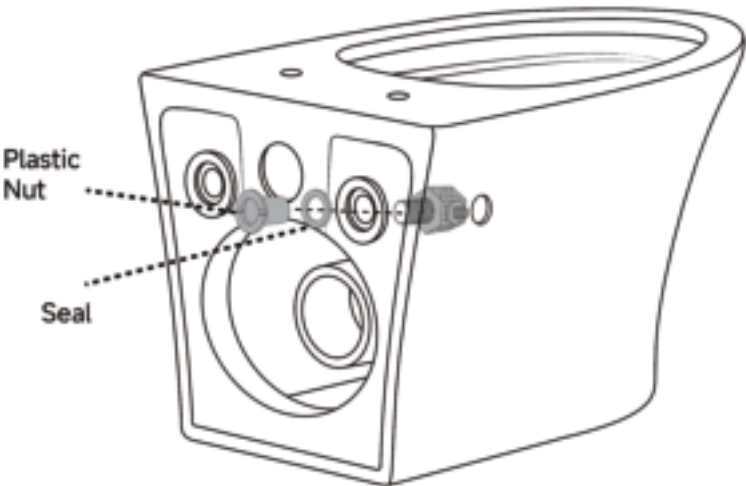
③ Insert the bracket into the bowl mounting hole and secure with seal and plastic nut
