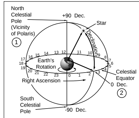
Fig. 25: Celestial Sphere.
