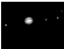
Fig. 33: Jupiter and its four largest moons. The moons can be observed in a different position every night.
