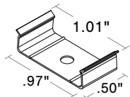
Stainless Steel Clip (SST-09)
