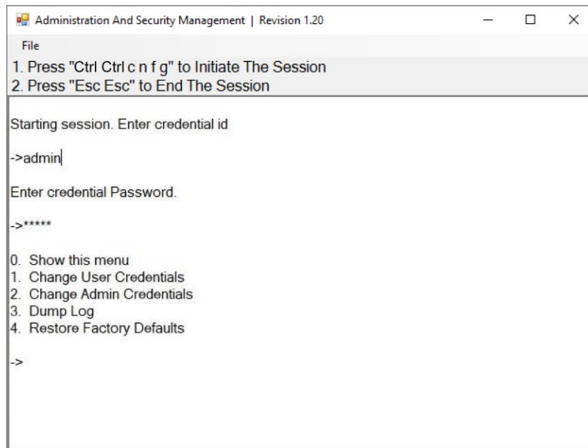
Figure 3: Administrator Log-in
