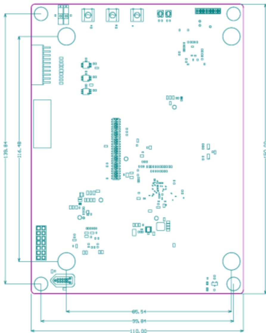
Figure 6. Board mechanical drawing (in millimeters)
