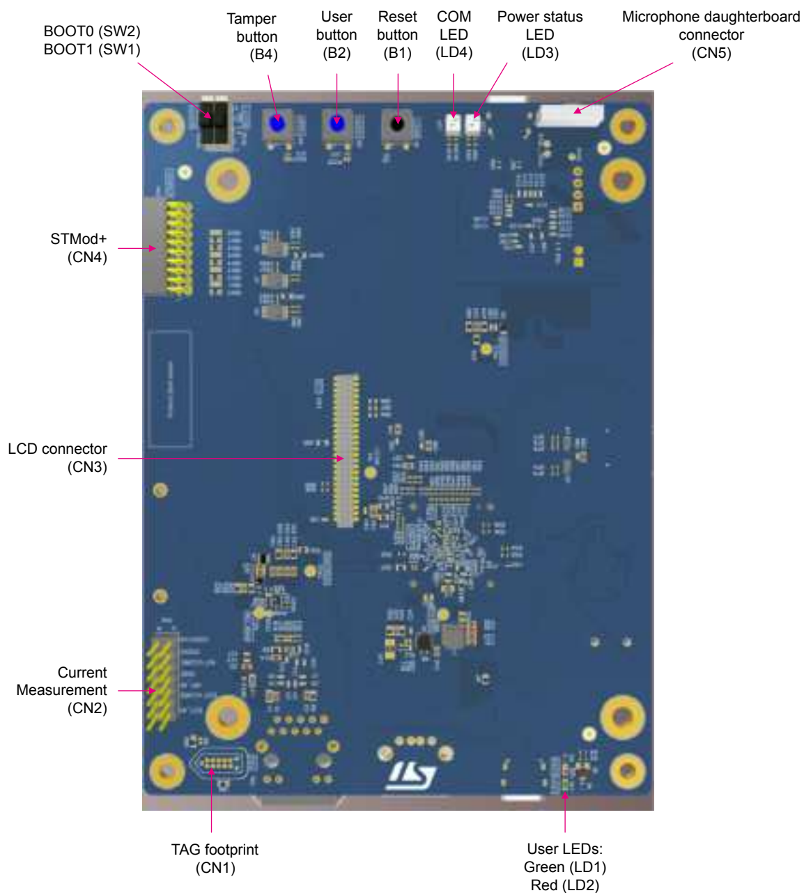
Figure 4. STM32N6570-DK PCB layout top view
