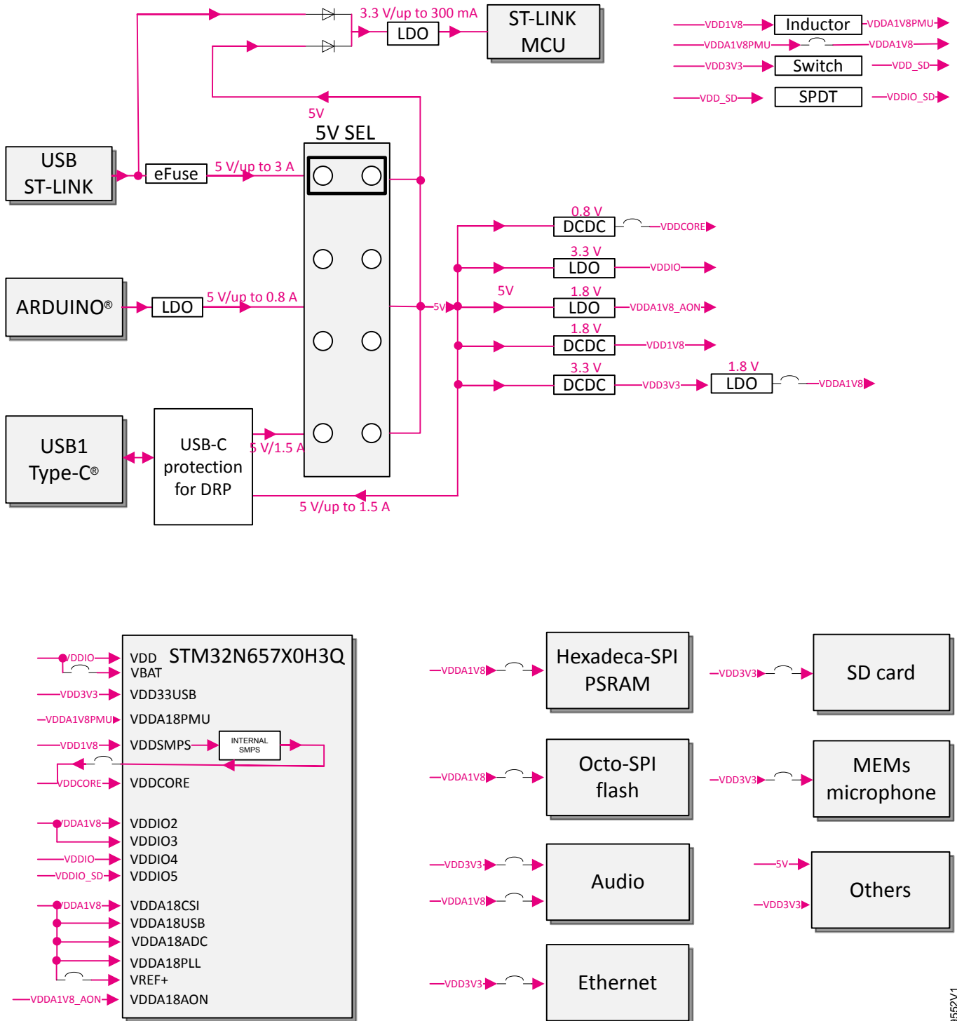
Figure 7. Power diagram
