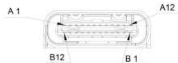
Figure 17. STLINK-V3EC connector (CN6) front view
