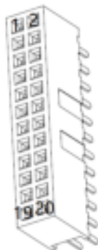
Figure 16. Microphone connector (CN5)
