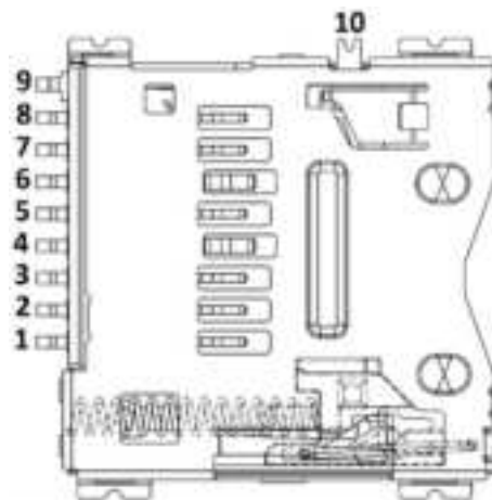
Figure 19. microSD™ connector (CN13) top view
