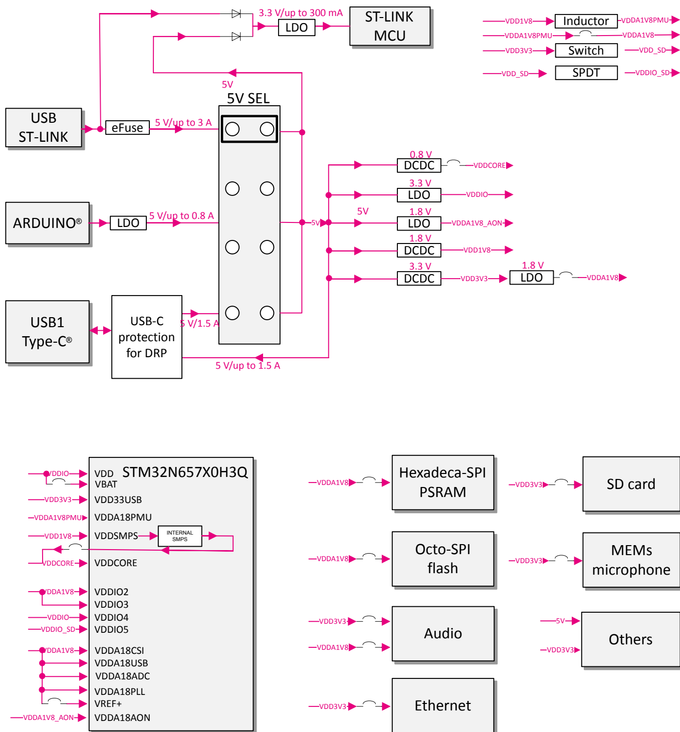
Figure 7. Power diagram
