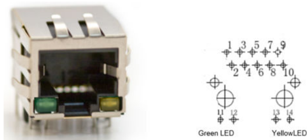
Figure 22. Ethernet RJ45 connector (CN16) front view
