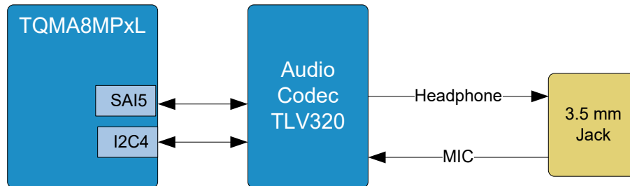
Figure 15: Block diagram audio interface
