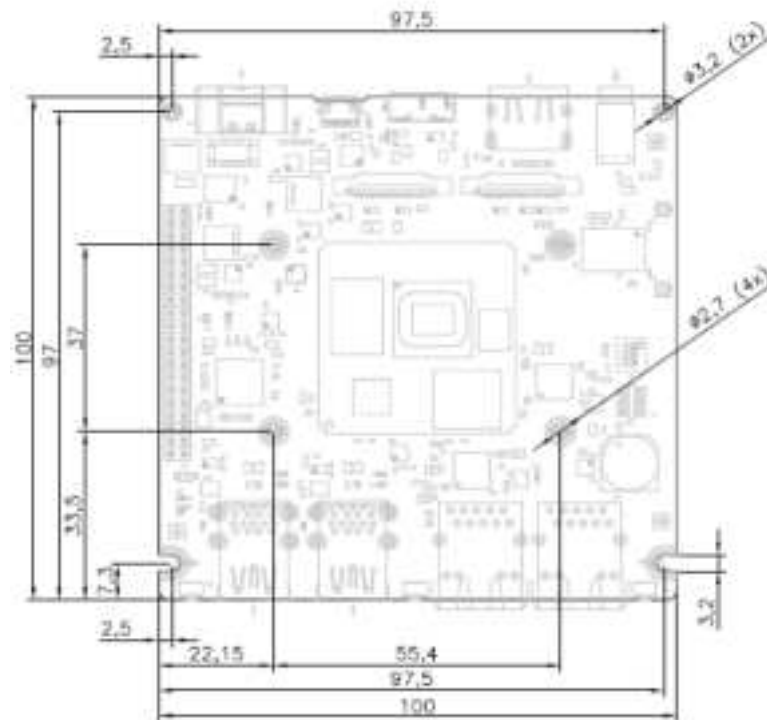
Figure 17: Dimensions MBa8MP-RAS314
