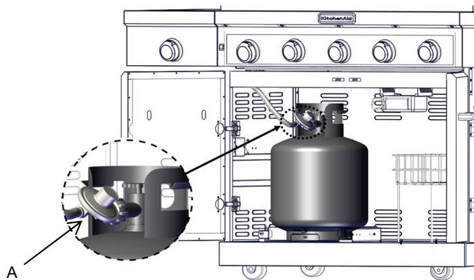
A. Gas pressure regulator/Hose assembly
