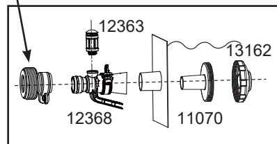
Adaptor B
