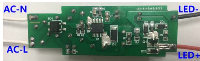
Figure 2: Bottom View
