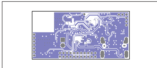
MAXSENSORBLE_EVKIT_B—Layer 7
