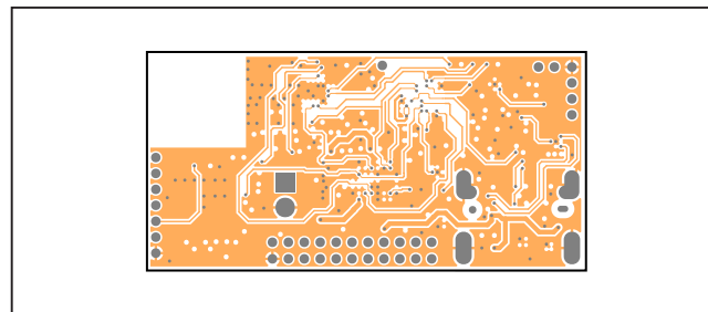
MAXSENSORBLE_EVKIT_B—Layer 5
