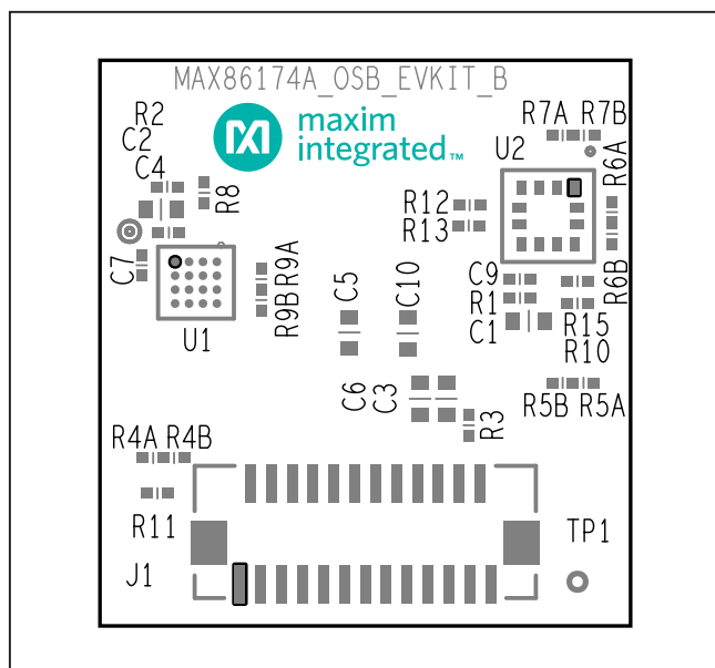
MAX86174A_OSB_EVKIT_B—Silkscreen Top
