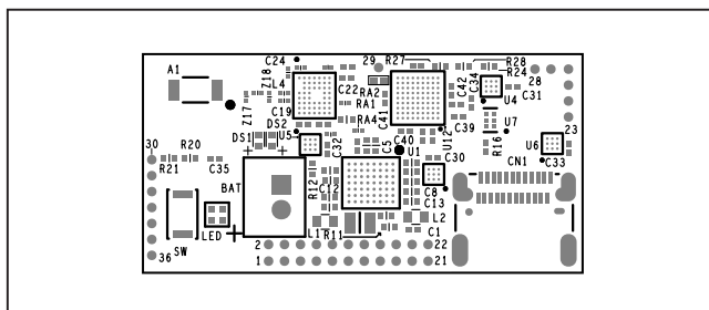
MAXSENSORBLE_EVKIT_B—Top Layer
