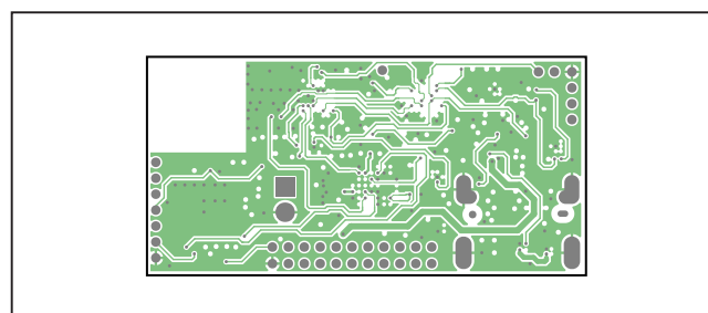
MAXSENSORBLE_EVKIT_B—Layer 3
