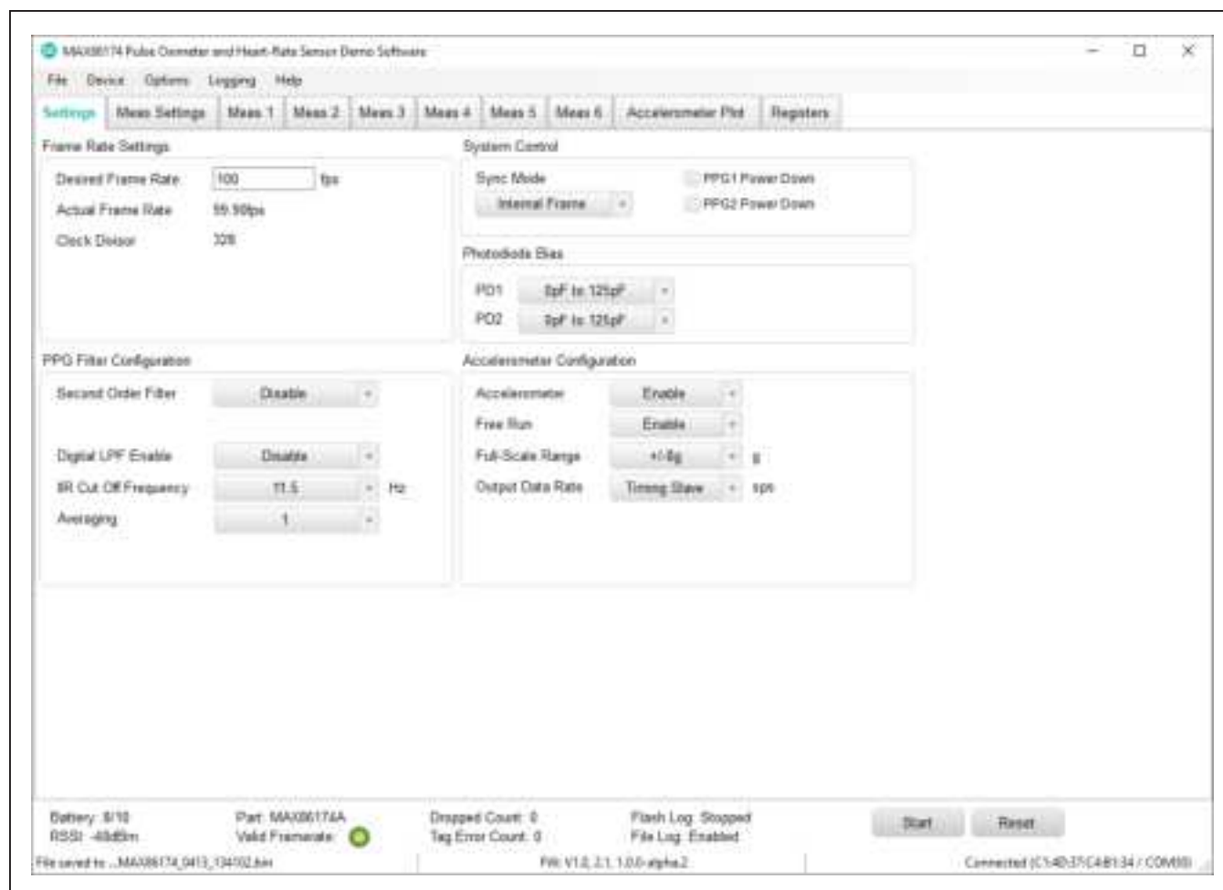
Figure 5. Settings Tab
