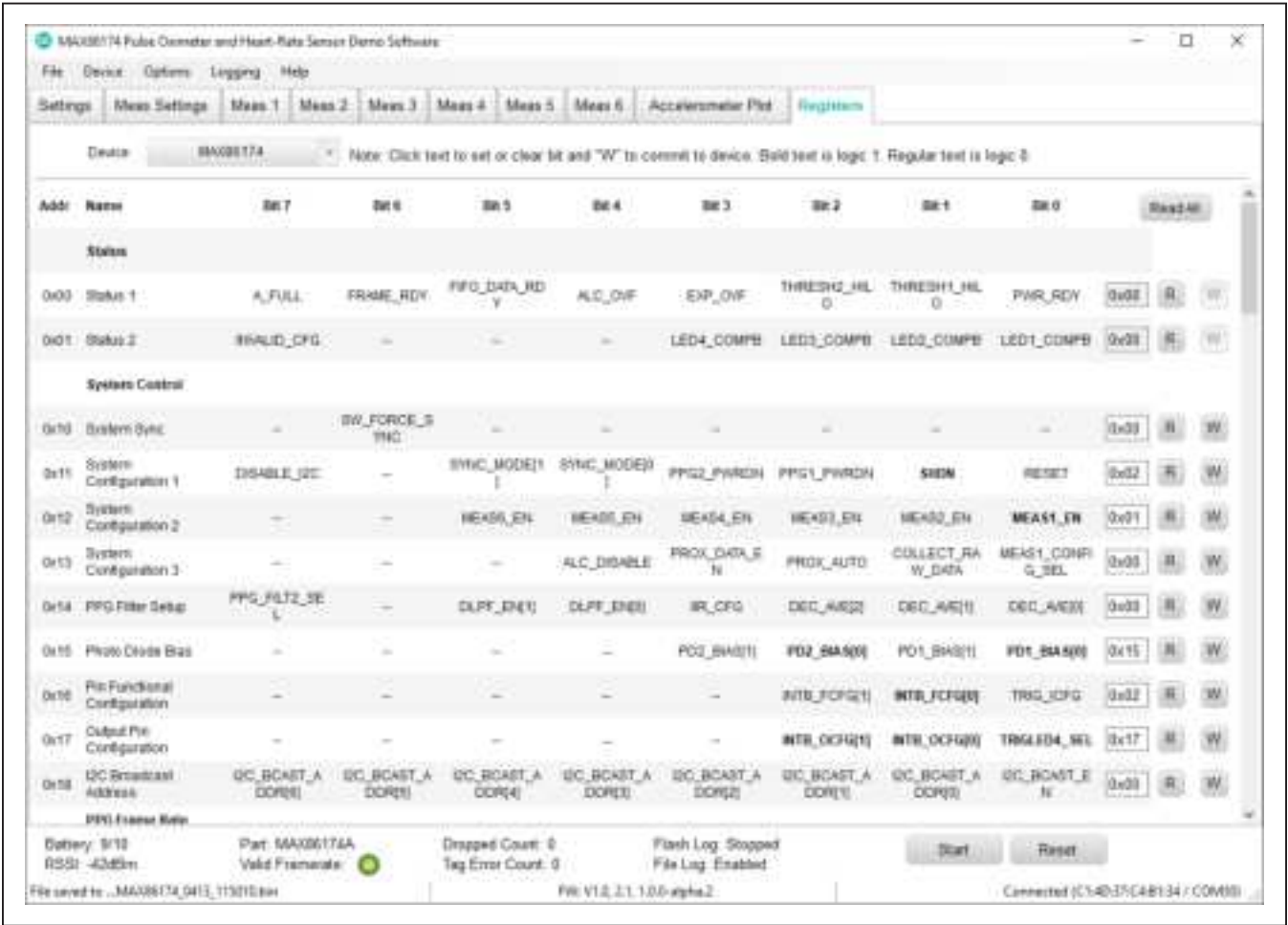
Figure 9. Registers Tab
