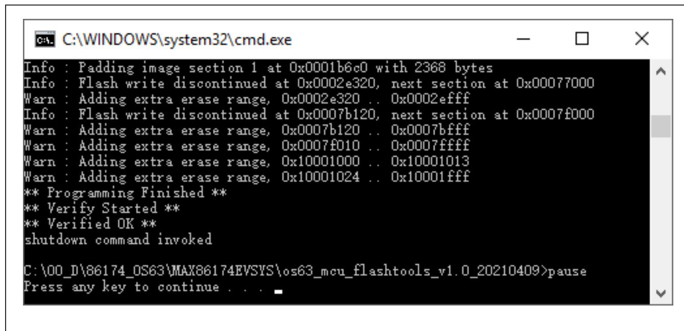
Figure 15. Command Prompt Display when Firmware Has Successfully Been Flashed
