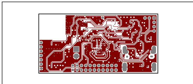
MAXSENSORBLE_EVKIT_B—Layer 6
