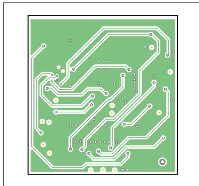
MAX86174A_OSB_EVKIT_B—Layer 3
