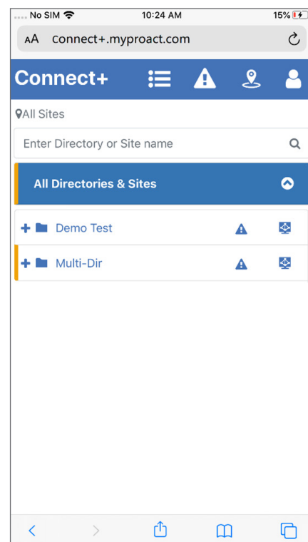
Connect+ UI
