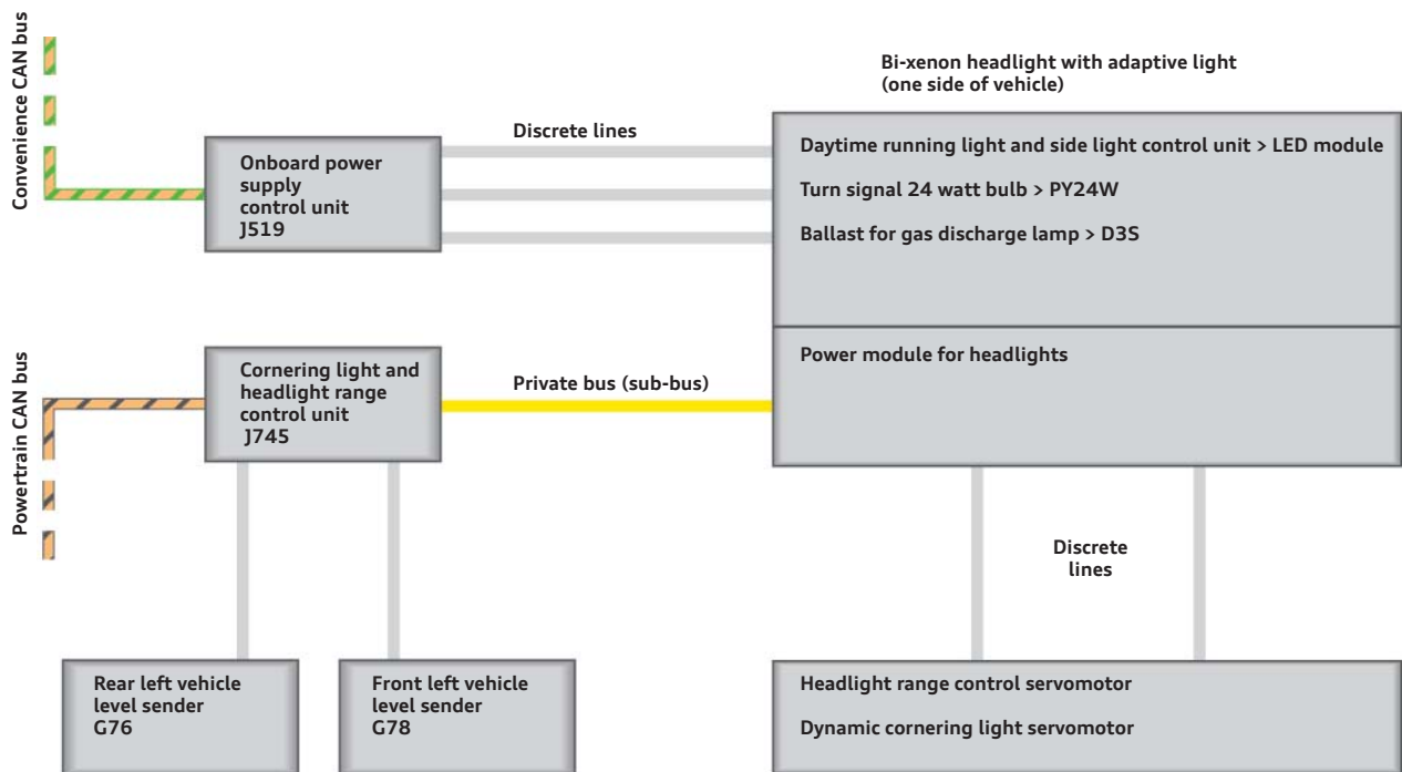
Schematic diagram of the activation mechanism for bi-xenon headlights with adaptive light
