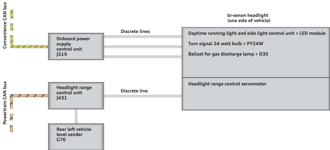
Schematic diagram of the activation mechanism for bi-xenon headlights
