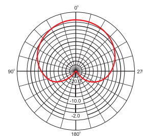
Cardioid at 1KHz
