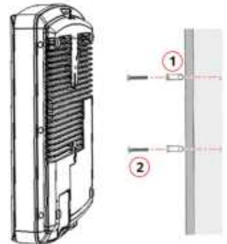
FIGURE 9 Flat Surface Mounting
