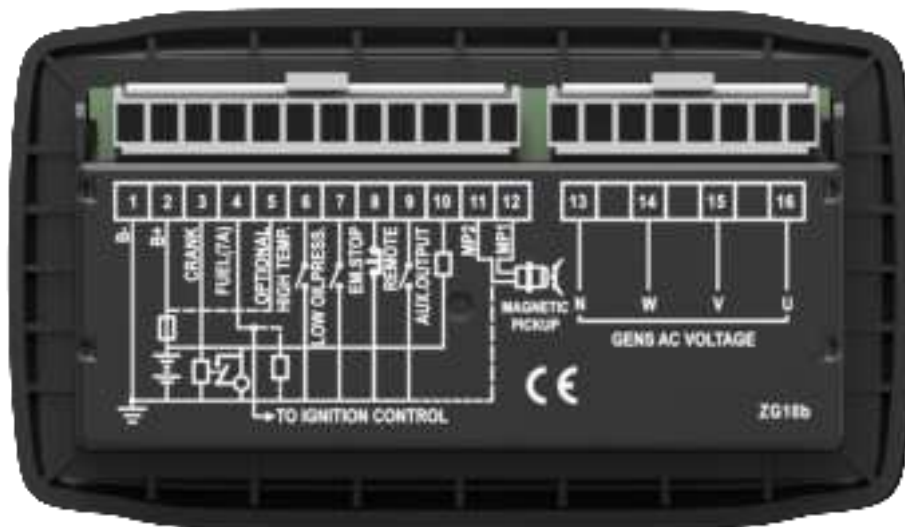
Fig.2 Rear Panel
