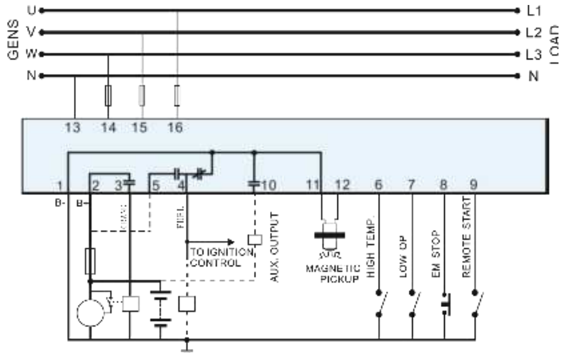
Fig.4 Typical Application
