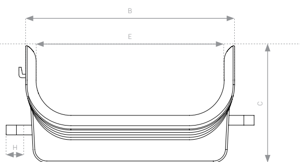
END VIEW
