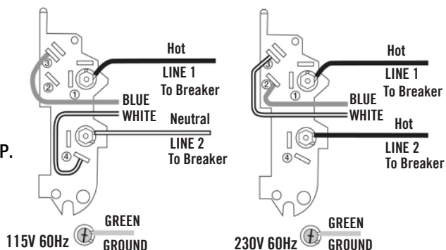
Wiring Diagram for EFLS10-HD
