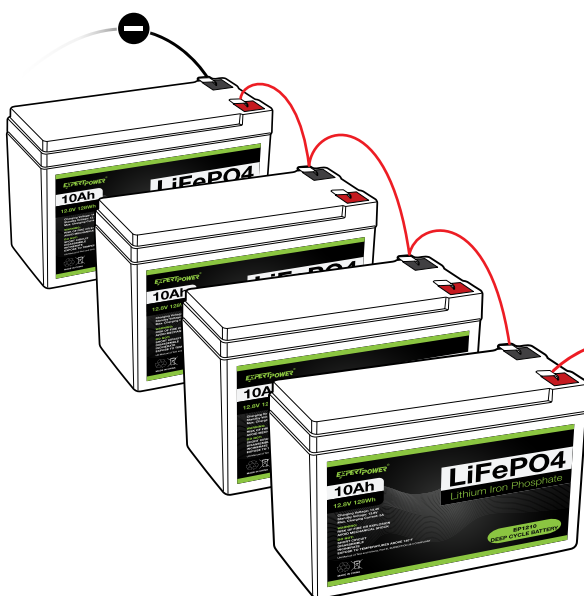
4 In Series - 48V 10Ah
