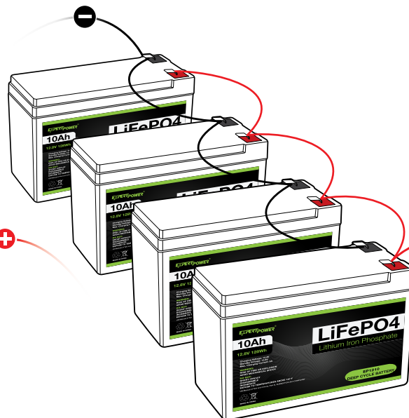
4 In Parallel - 12V 40Ah
