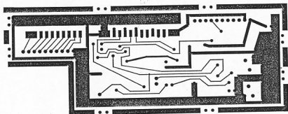
AR2002 CPU/LCD UNIT COMPONENT SIDE
