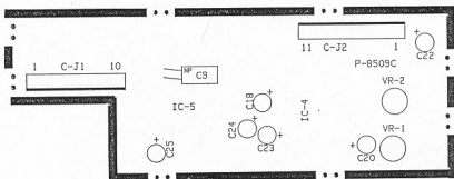
AR2002 CPU/LCD UNIT COMPONENT LOCATION
