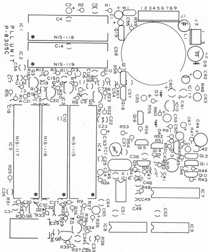
PLL UNIT COMPONENT LOCATION FOR THE AR2002 SERIAL NUMBERS UP TO 1500.
