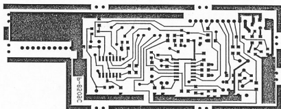
AR2002 CPU/LCD UNIT SOLDER FOIL SIDE
