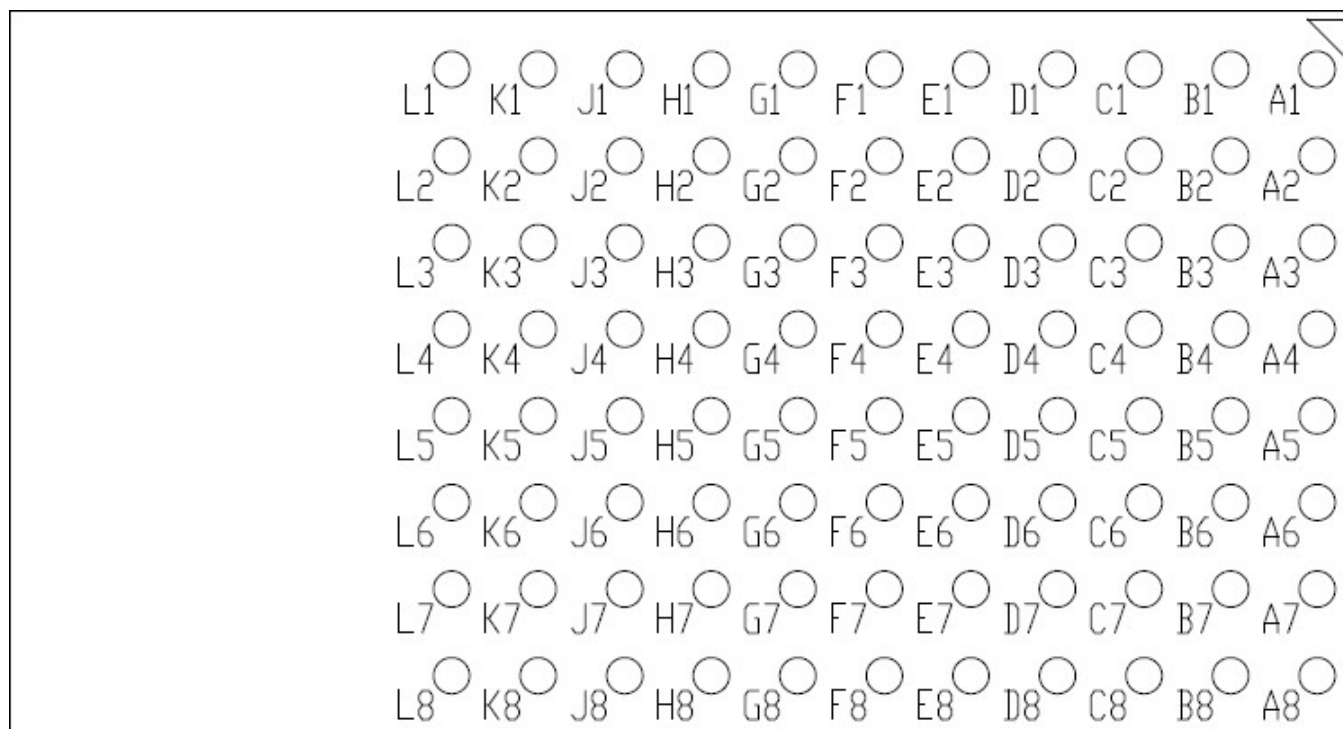
AW-CU570 Pin Map (Top View)
