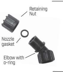
6-8148 Nozzle Kit
