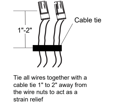
DRAWING 3- Cable tie diagram
