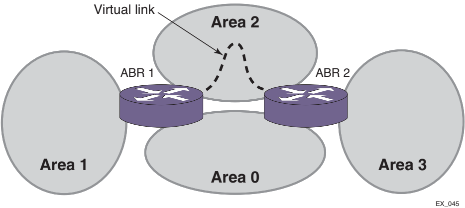
Figure 77. Virtual Link Providing Redundancy
