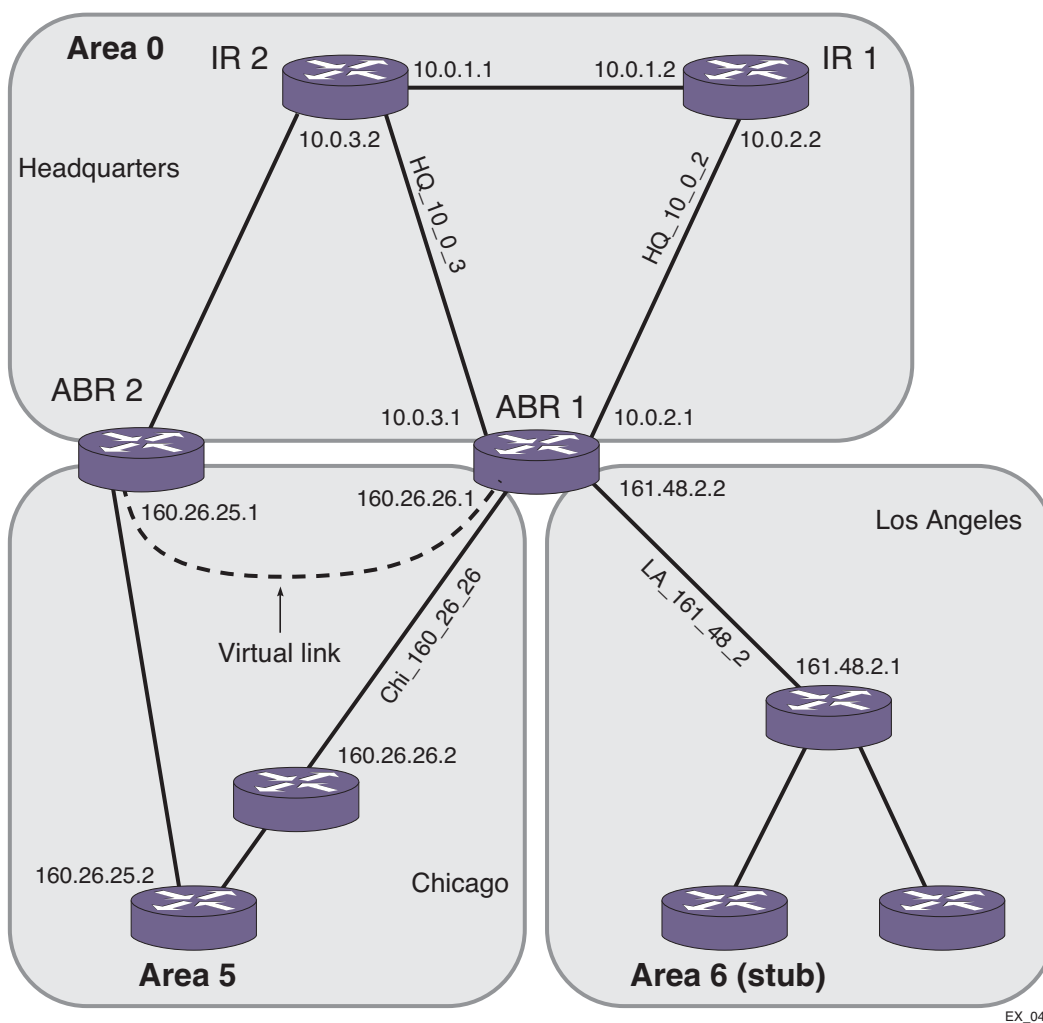
Figure 75. OSPF Configuration Example
