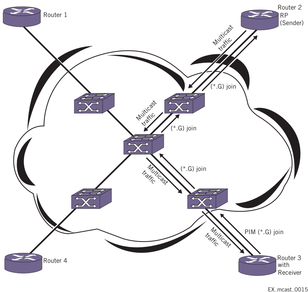
Figure 84. Multicast With PIM Snooping
