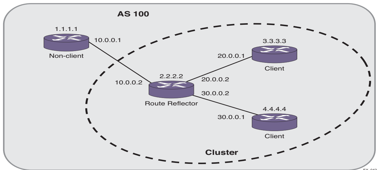
Figure 80. Route Reflectors
