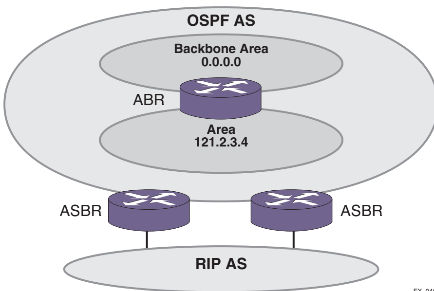
Figure 70. Route Redistribution
