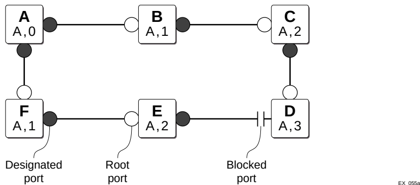
Figure 42. Initial Network Configuration
