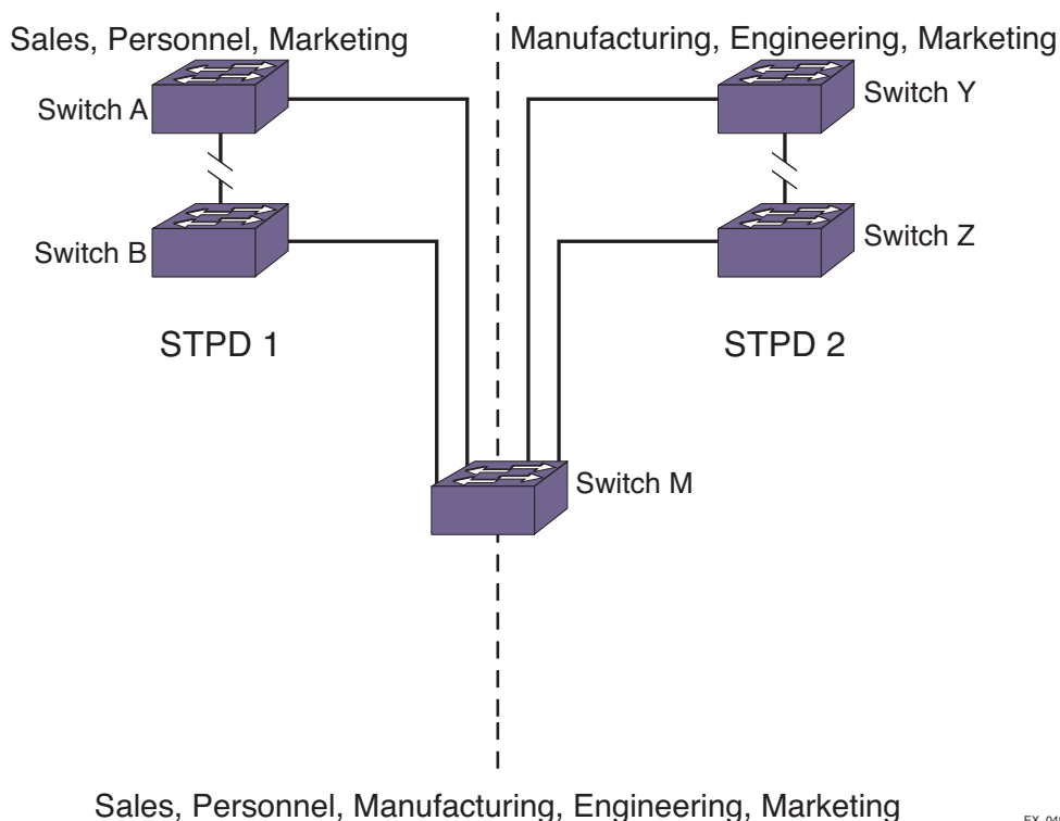
Figure 35. Multiple STPDs
