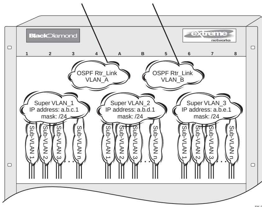
Figure 66. VLAN aggregation
