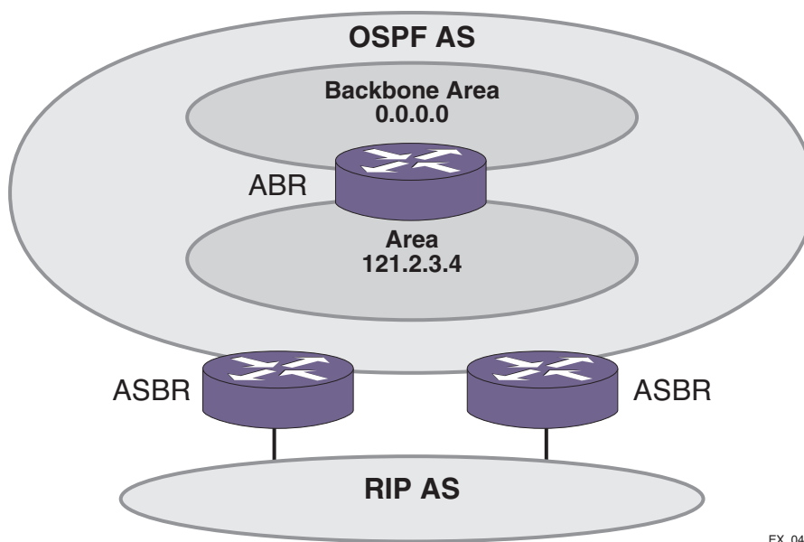
Figure 74. Route Redistribution
