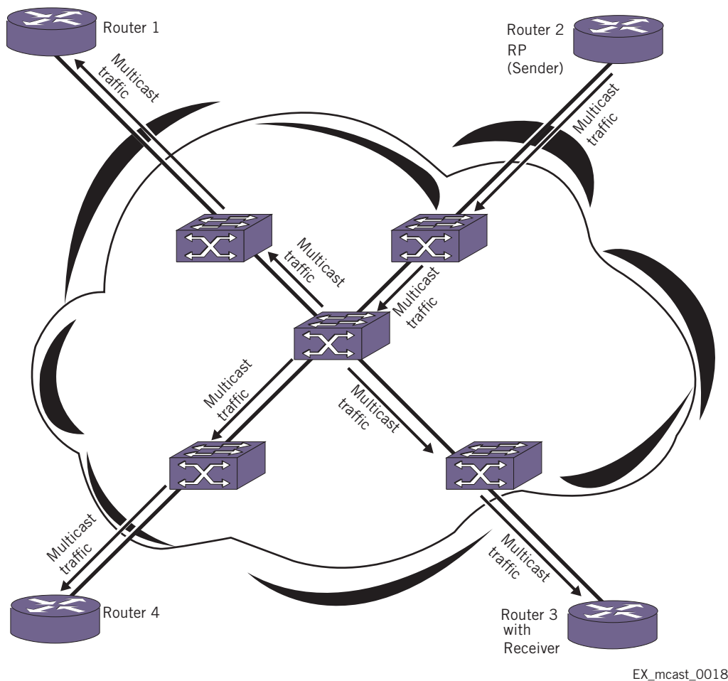
Figure 83. Multicast Without PIM Snooping
