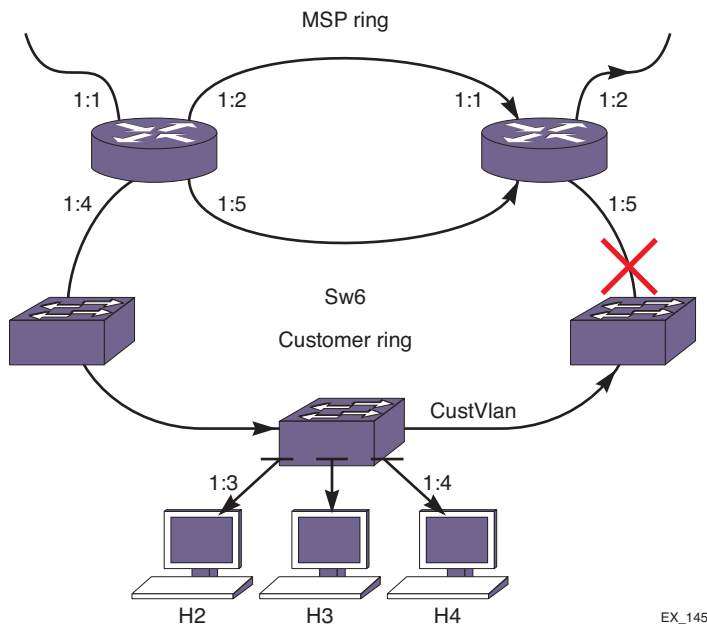
Figure 91. Inter-Multicast VLAN Forwarding
