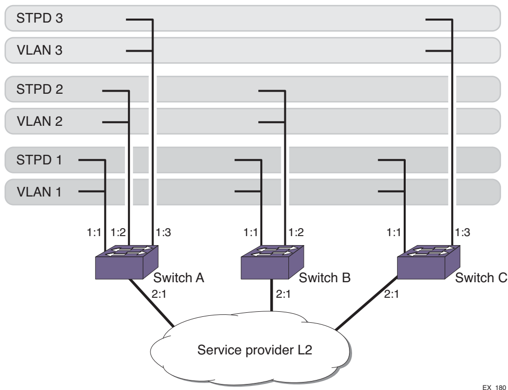
Figure 34. Sample Network Using STPD BPDUs Tunneling
