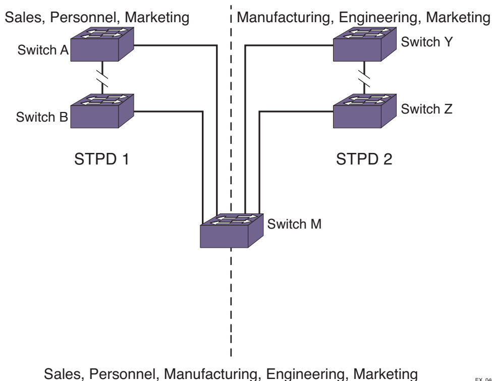
Figure 57. RSTP Example
