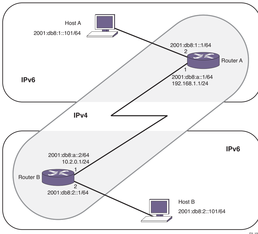
Figure 68. 6in4 Tunnel Example
