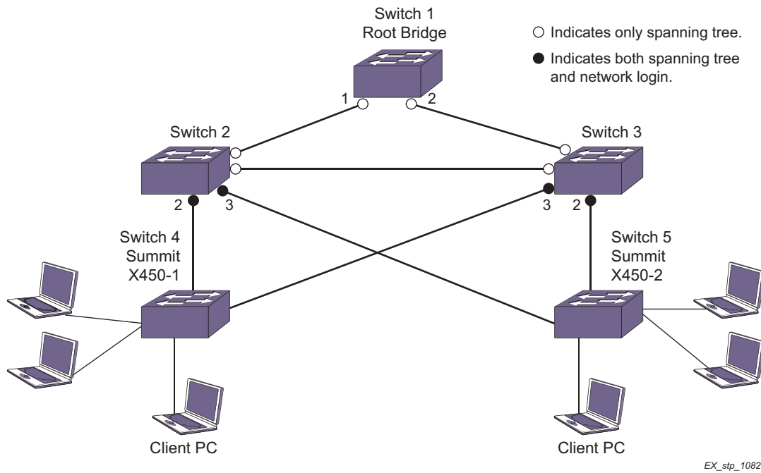
Figure 54. STP and Network Login Enabled
