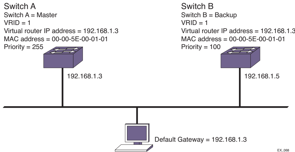
Figure 59. Simple VRRP Network
