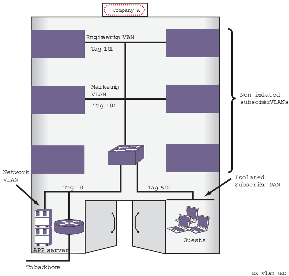
Figure 12. VLAN Isolation Application
