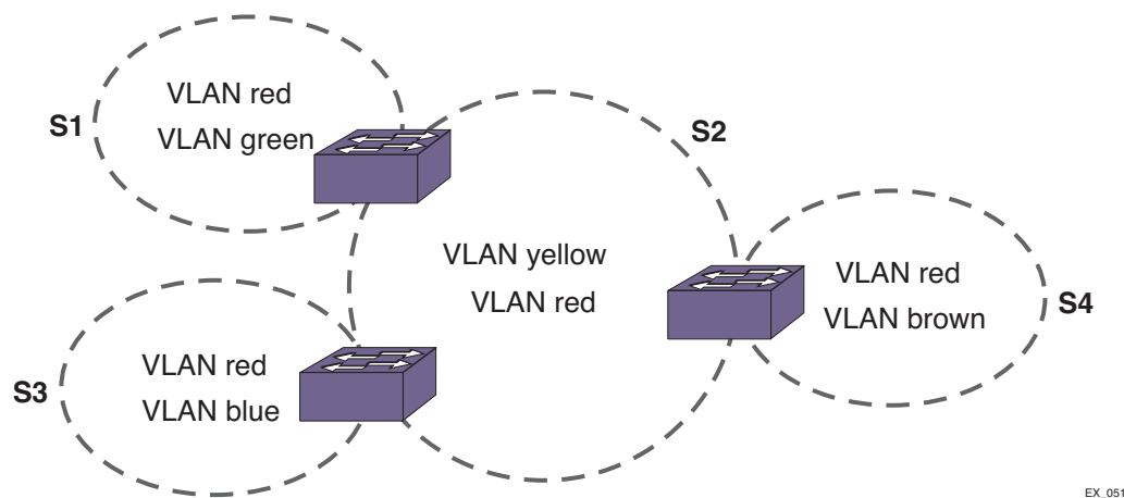
Figure 38. VLANs Spanning Multiple STPDs
