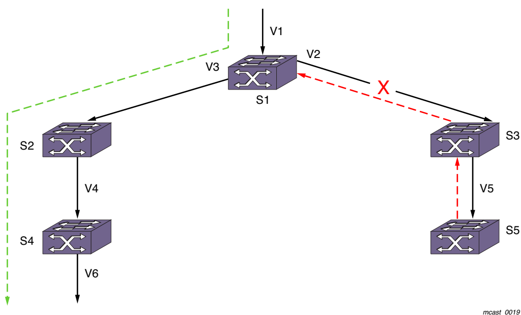
Figure 82. PIM-DM Operation
