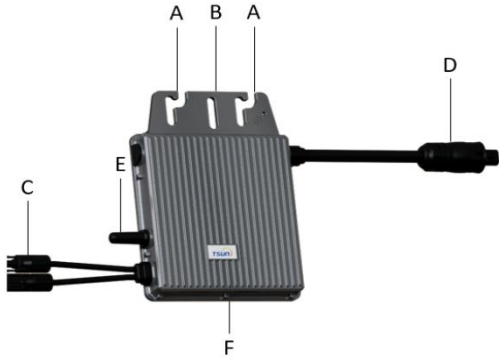
Balcony Microinverter(1PV)
