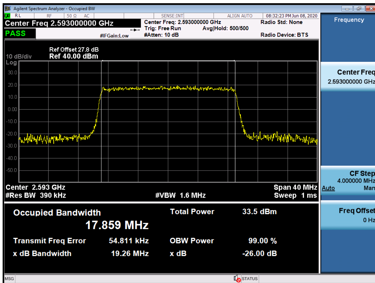
Occupied Bandwidth Plot (20 MHz Ch.40620 16-QAM RB 100) (POWER CLASS 2)
