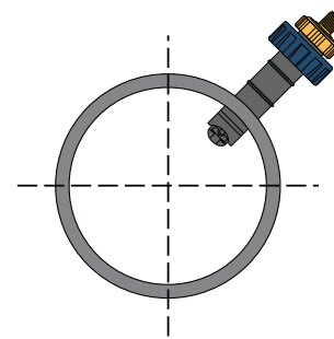
Preferred installation if SEDIMENT* or AIR BUBBLES may be present
