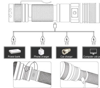
Figure 1.1 Power supply
