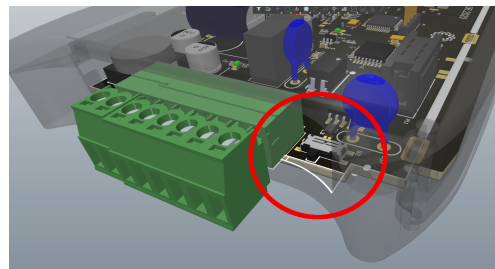
Fig. 6: Termination switch.
