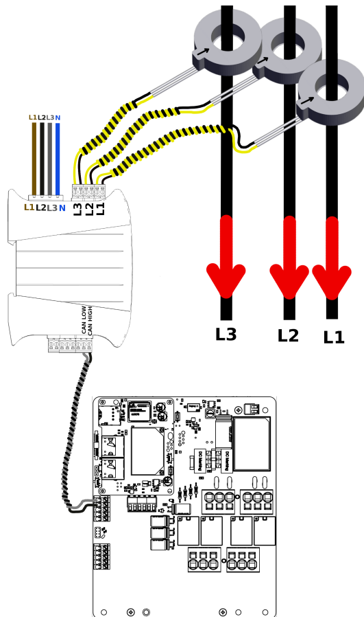
Fig. 5: Energy Guard 3-phase variant connection diagram.
