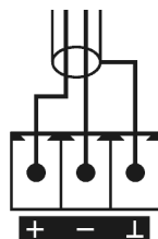
Balanced Wiring
