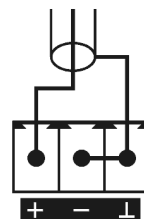
Unbalanced Wiring
