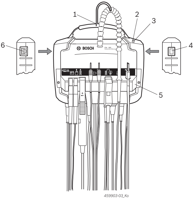
Fig. 1: Front view FSA 500 1 Carrying strap with hook 2 LED A: Status light 3 LED B: Charge indicator 4 On/Off switch 5 Sensor bracket 6 USB port
