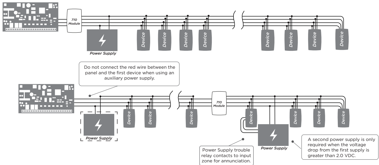
Figure 7: Installing Optional Power Supplies
