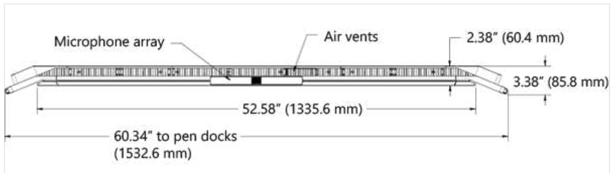
Front view of 55" Surface Hub
