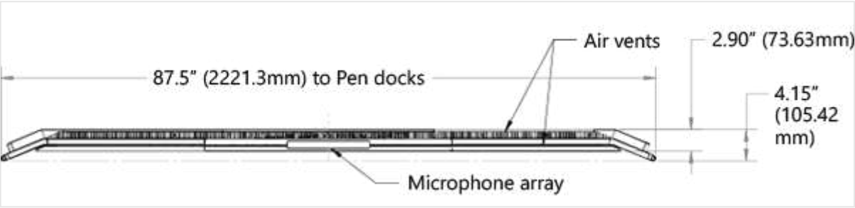
Front view of 84" Surface Hub
