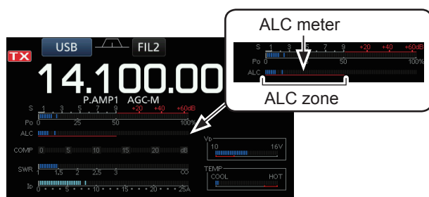
Multi-function meter
