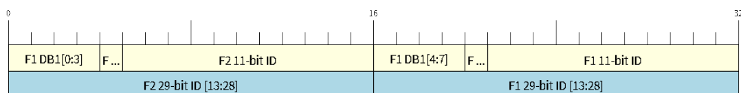
图 37: Bit layout of dual filter mode (Right side MSBit)
