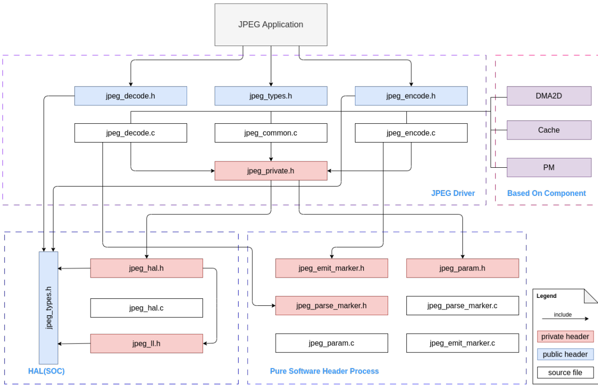
图 33: JPEG driver file structure
