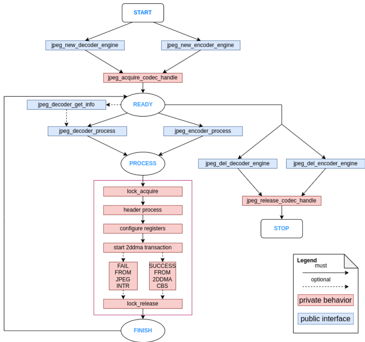
图 25: JPEG finite state machine
