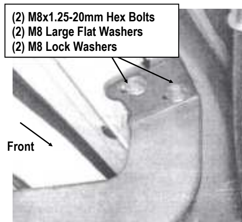
(Fig 3) Driver Side Rear Mounting Bracket Installed
