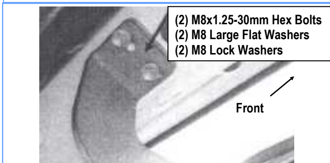
(Fig 2) Driver Side Center Mounting Bracket Installed
