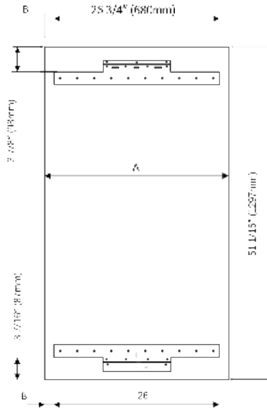
30" & 36" BUILT-IN BOTTOM MOUNT
