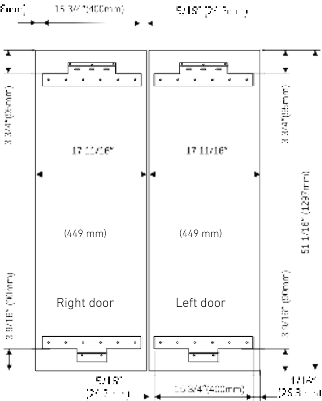
36" BUILT-IN FRENCH DOOR
